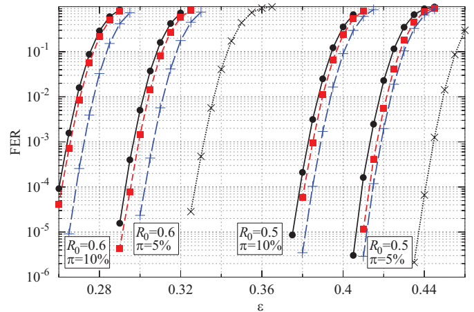
Fig. 2. FER over the BEC with crossover probability \epsilon for different intentional puncturing strategies. Two LDPC codes with coding rates R_0 = 0.5 and R_0 = 0.6 , and two different proportions of punctured symbols, \pi = 5\% and \pi = 10\% were used. See inset in Fig. 1 for symbols and line-styles.
