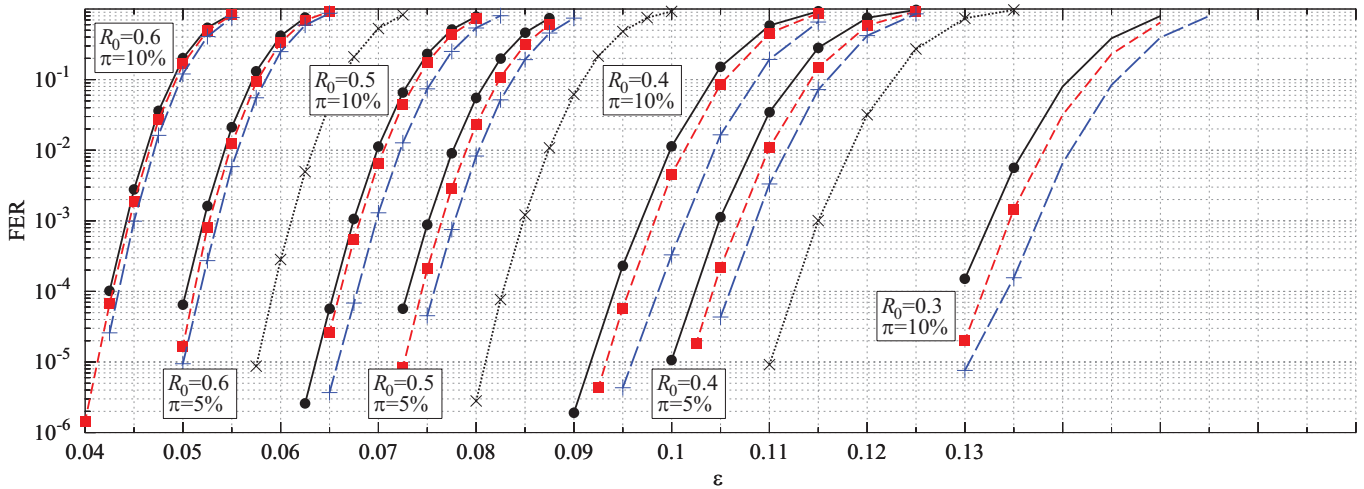
Fig. 3. FER over the BSC with crossover a probability \varepsilon for several LDPC codes with coding rates R_0 = 0.3 , R_0 = 0.4 , R_0 = 0.5 and R_0 = 0.6 , and two different proportions of punctured symbols, \pi = 5\% and \pi = 10\% .
